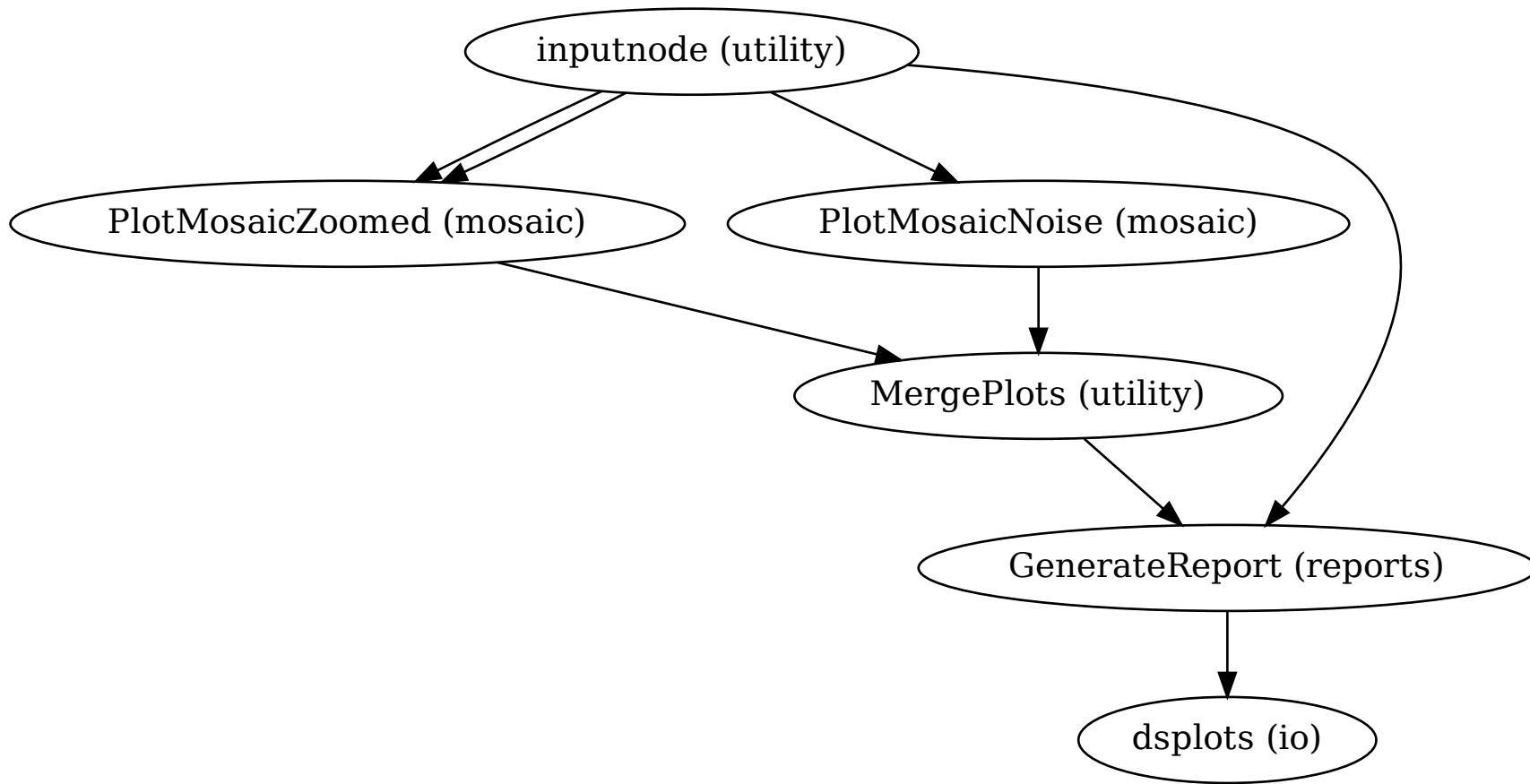
ReportsWorkflow
